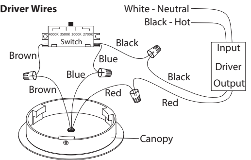
Fig. 4 Driver Wires
