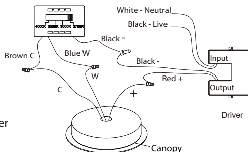
Fig.4 Driver Wires
