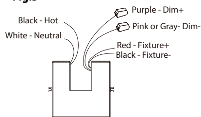
Fig.4 Driver Wires
